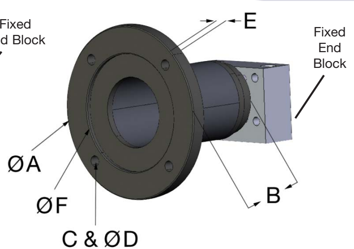
B14 Flange Configuration
