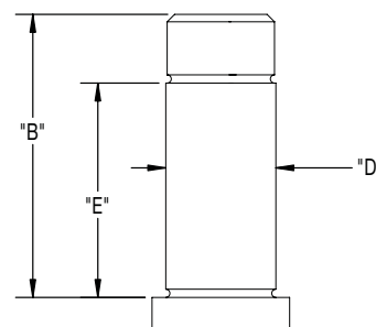
Type 3B - without Drive End
