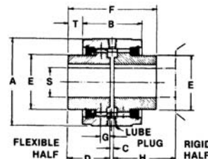
Flex—Rigid Coupling
