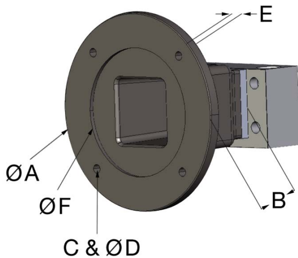
B5 Flange Configuration
